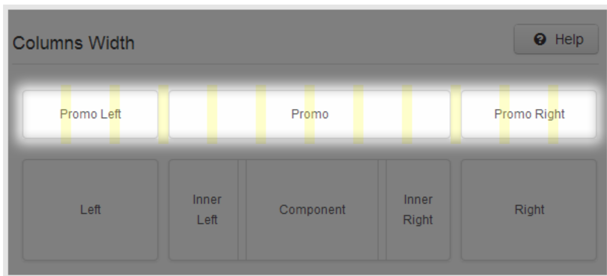
12 Bootstrap grids
