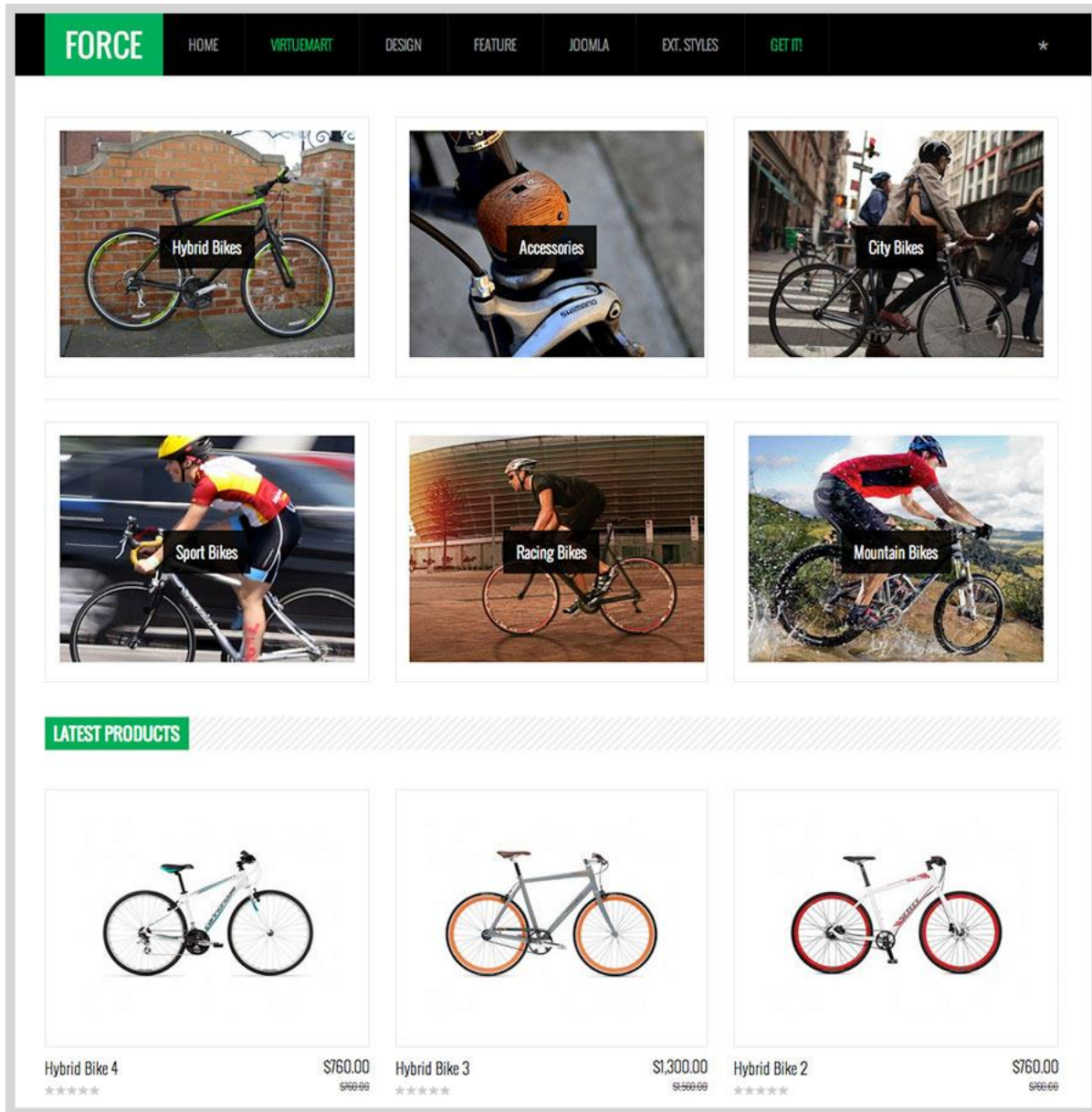
VirtueMart Component
